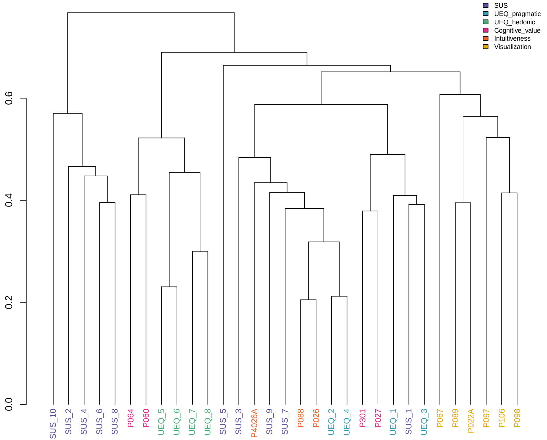
Hierarchical clustering of items (distance = 1 - r)
